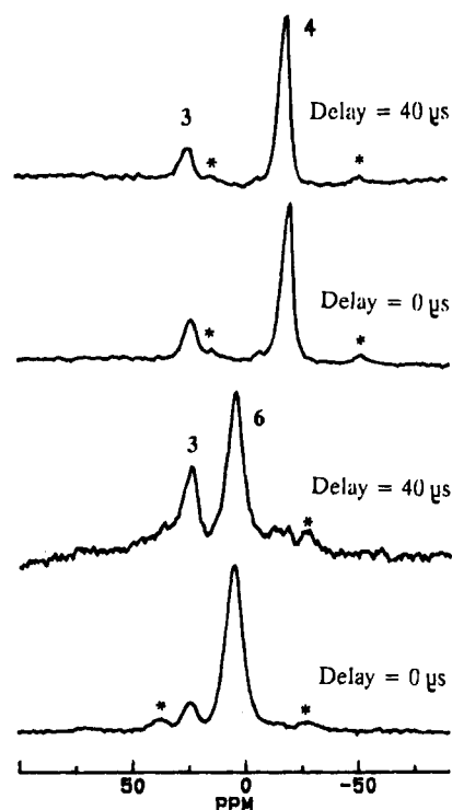
Figure 6. Dipolar dephasing experiments of original (top two spectra) and protonated (bottom two spectra) silica 4 , containing little 3 , with the given delays: 3 = side product; 4 = silica-immobilized phosphine 1 ; 6 = phosphonium salt of 4 . Asterisks denote rotational sidebands of signals 4 and 6 .
