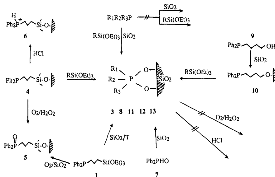
Scheme 2. Overview of the Main Results of Section II a
