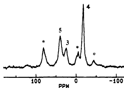
Figure 2. 121.5 MHz 31 P CP/MAS NMR spectrum of silica after immobilization of phosphine 1 in air: 3 = side product; 4 = immobilized phosphine; 5 = phosphine oxide. Asterisks denote rotational sidebands of signal 5.
