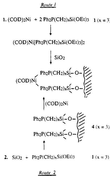
Scheme 1. Two Possible Strategies in Order to Immobilize a Transition Metal Complex a
