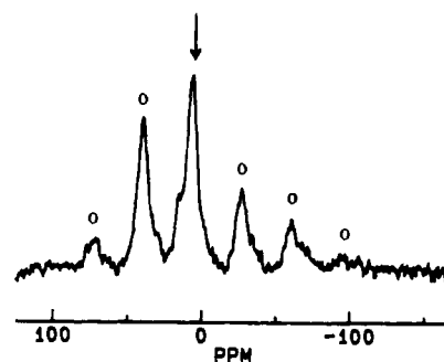
Figure 1. 121.5 MHz 31 P CP/MAS NMR spectrum of diphenylphosphinic acid immobilized on silica. The arrow denotes the isotropic line; the circles, rotational sidebands.
