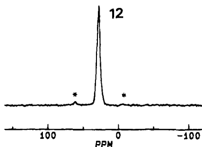
Figure 8. 121.5 MHz ^{31}\text{P} CP/MAS NMR spectrum of \text{Ph}_2\text{PEt}/\text{RSi}(\text{OEt})_3 -modified silica 12 . Asterisks denote rotational sidebands.
