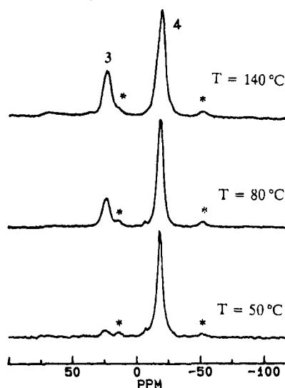
Figure 4. 121.5 MHz 31 P CP/MAS NMR spectrum of silica, modified with phosphine 1 at the given temperatures: 3 = side product; 4 = silica-immobilized phosphine 1. Asterisks denote rotational sidebands of signal 4.
