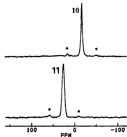
Figure 7. 121.5 MHz ^{31}\text{P} CP/MAS NMR spectra of modified silica: top trace, immobilized (4-hydroxybutyl)diphenylphosphine ( 10 ); bottom trace, P(V) species 11 , prepared by treatment of 10 with \text{RSi}(\text{OEt})_3 . Asterisks denote rotational sidebands.
