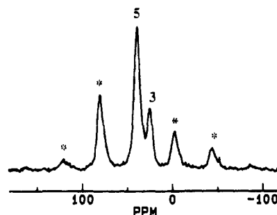
Figure 3. 121.5 MHz 31 P CP/MAS NMR spectrum of phosphine-modified silica 4, containing some side product 3, after oxidation with H 2 O 2 : 3 = side product; 5 = phosphine oxide. Asterisks denote rotational sidebands of signal 5.
