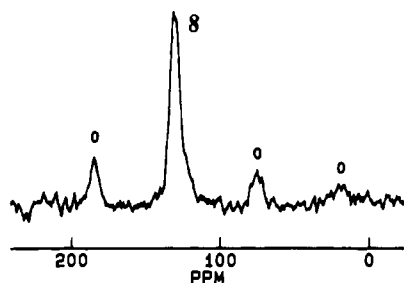
Figure 5. 75.5 MHz ^{13}\text{C} CP/MAS NMR spectrum of silica 8 , prepared by reaction of silica with diphenylphosphine oxide ( 7 ). Circles denote rotational sidebands of the phenyl resonance 8 .
